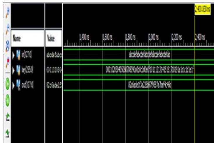
Fig 7 Encryption process
