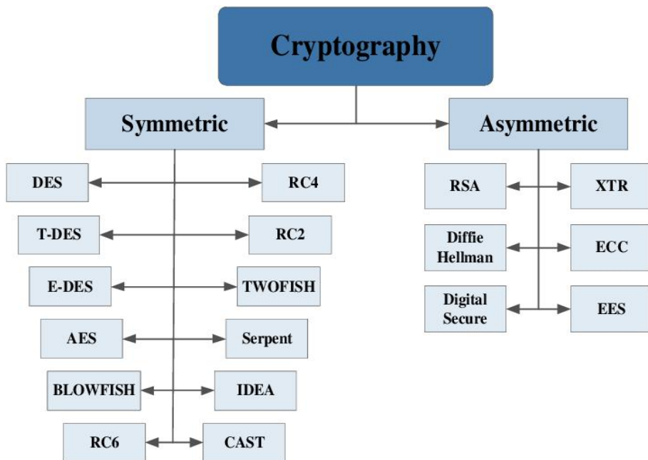
Fig 3 Cryptography stages
