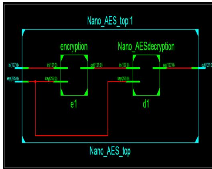
Fig 6 RTL view of Encryption and Decryption Process
