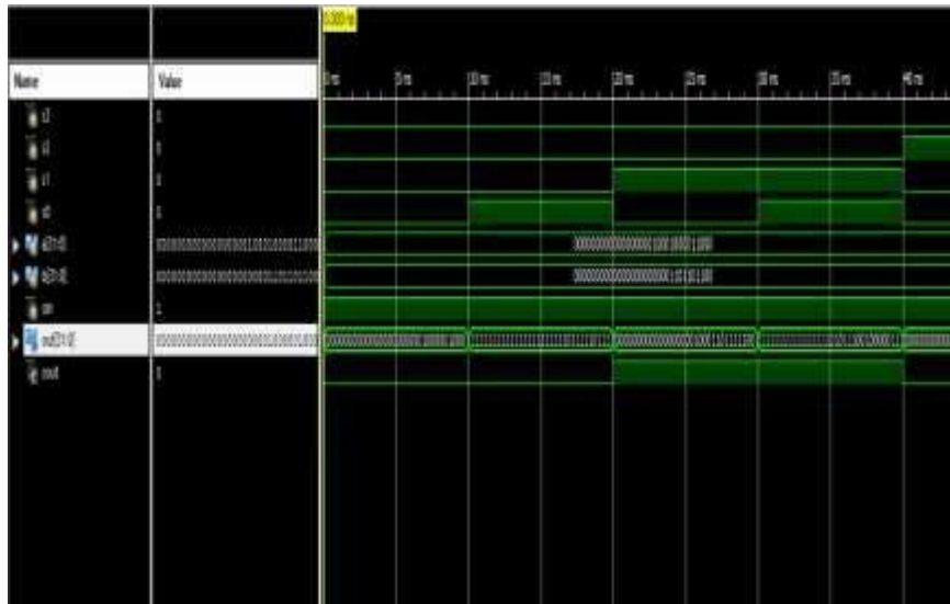
Fig. 6: OUTPUT WAVEFORM OF LOGICAL OPERATIONS
