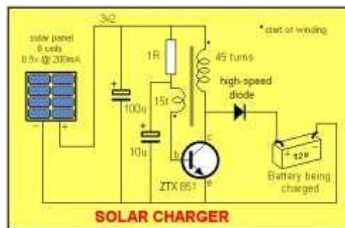
Fig 8. Solar Charger
