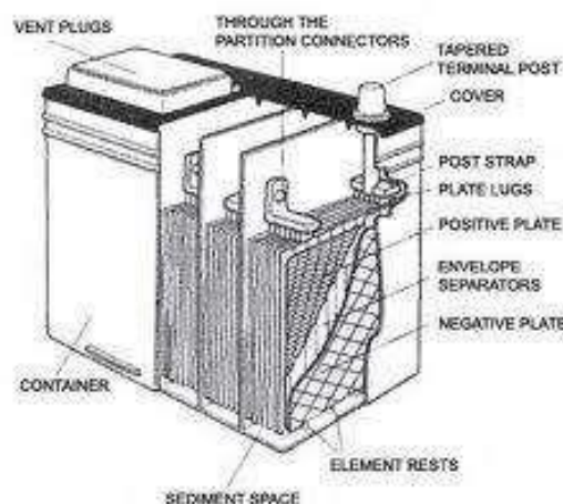
Fig .6. Lead Acid Battery
