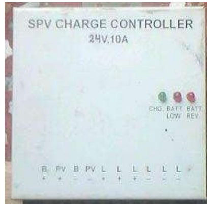
Fig 5 Solar charge controller unit
