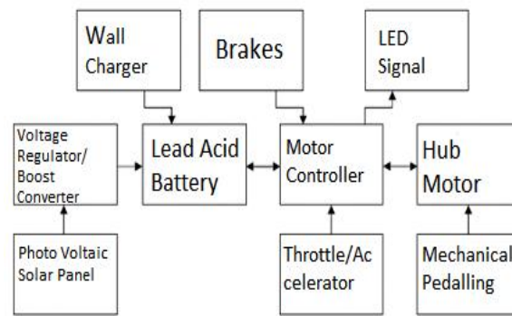
Fig 2 Basic block diagram of solar e bicycle
