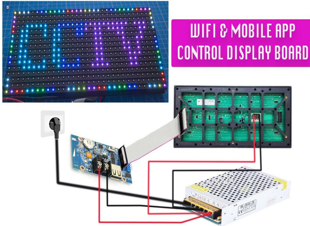
Figure 5 Single module display
