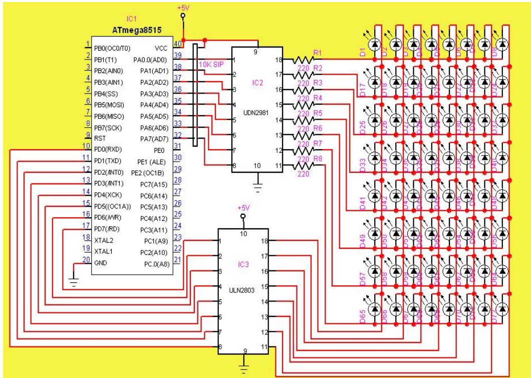
Fig 4 Circuit Diagram
